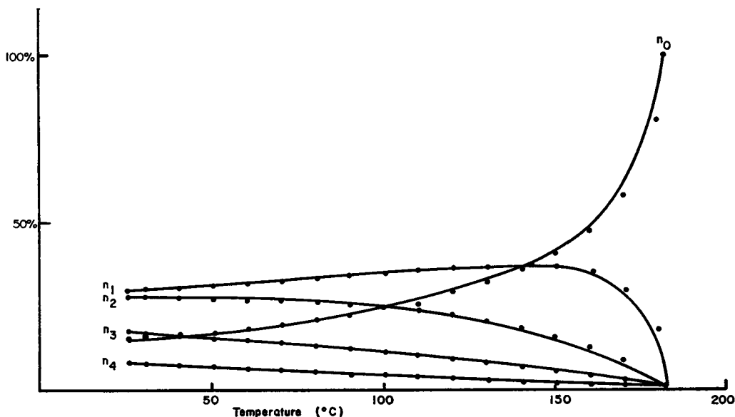
FIGURE 7 n_i , the number of i -type bonded water in a unit volume, as a function of temperature for a completely dried sample (zero water content; kept for 24 hr at 130°C).
